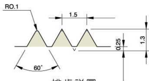
排齒詳圖 Drawing of Serration
